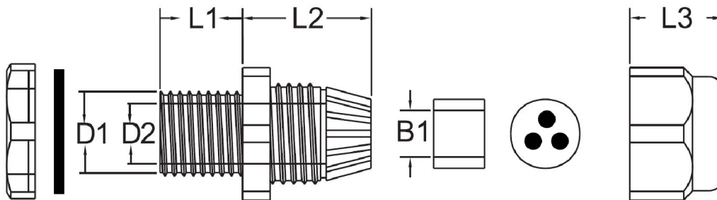
Multi Hole NPT Gland Specs (mm)
