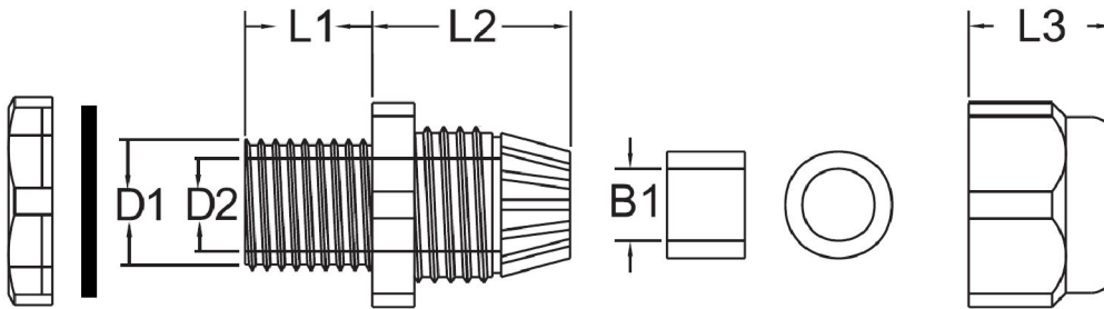
Metric Gland Specs (mm)
